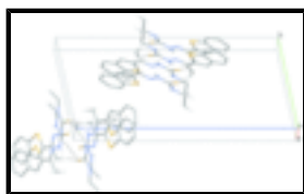
Fig. 3. C—H... \pi interactions between dimers in the title compound. Cg1 is the centroid of the S1A/C1A/C2A/C3A/C8A ring and Cg2 that of the S1B/C1B/C2B/C3B/C8B ring. H... Cg interactions are drawn as dotted lines and hydrogen bonds as dashed lines. H atoms not involved in these interactions and atoms of one of the disorder components have been omitted for clarity.
